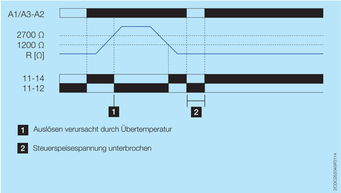
CM-MSS.12, CM-MSS.13
