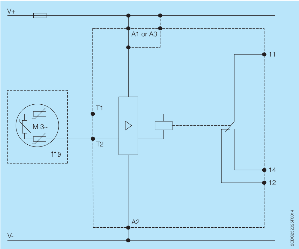
CM-MSS.13
