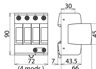
Dimension drawing DG M TNS ACI 275 FM
