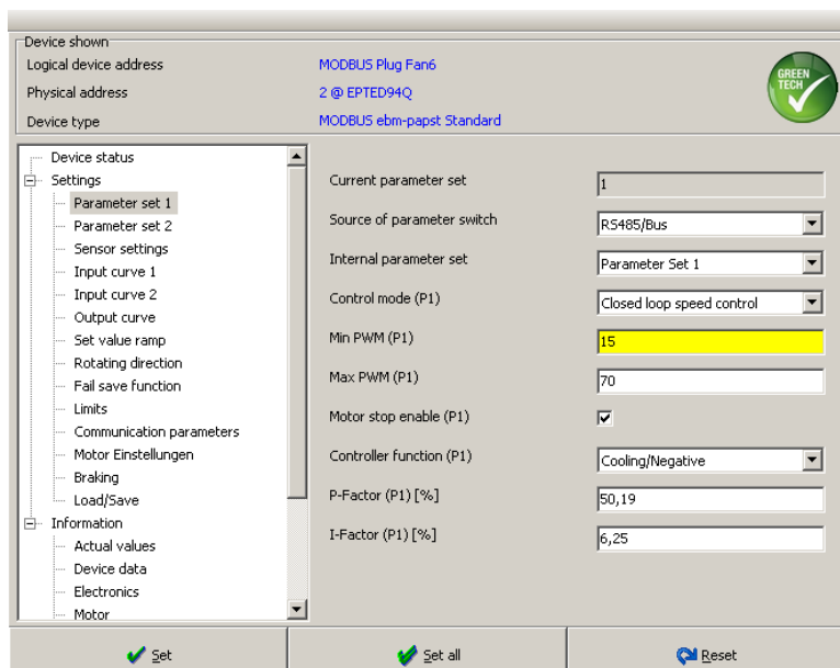
Fig. 14: Minimum and maximum PWM signal
