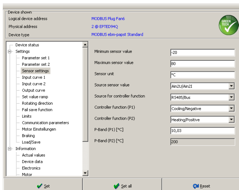
Fig. 11: Control function
