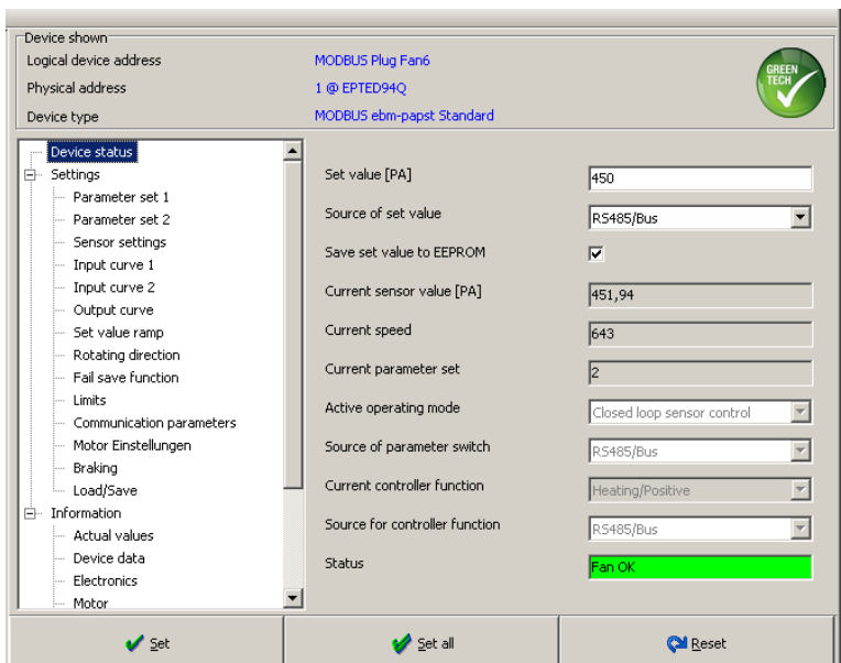
Fig. 60: digital setting of values for parameter set 2, differential pressure 450 Pa, enter set value for night switching
