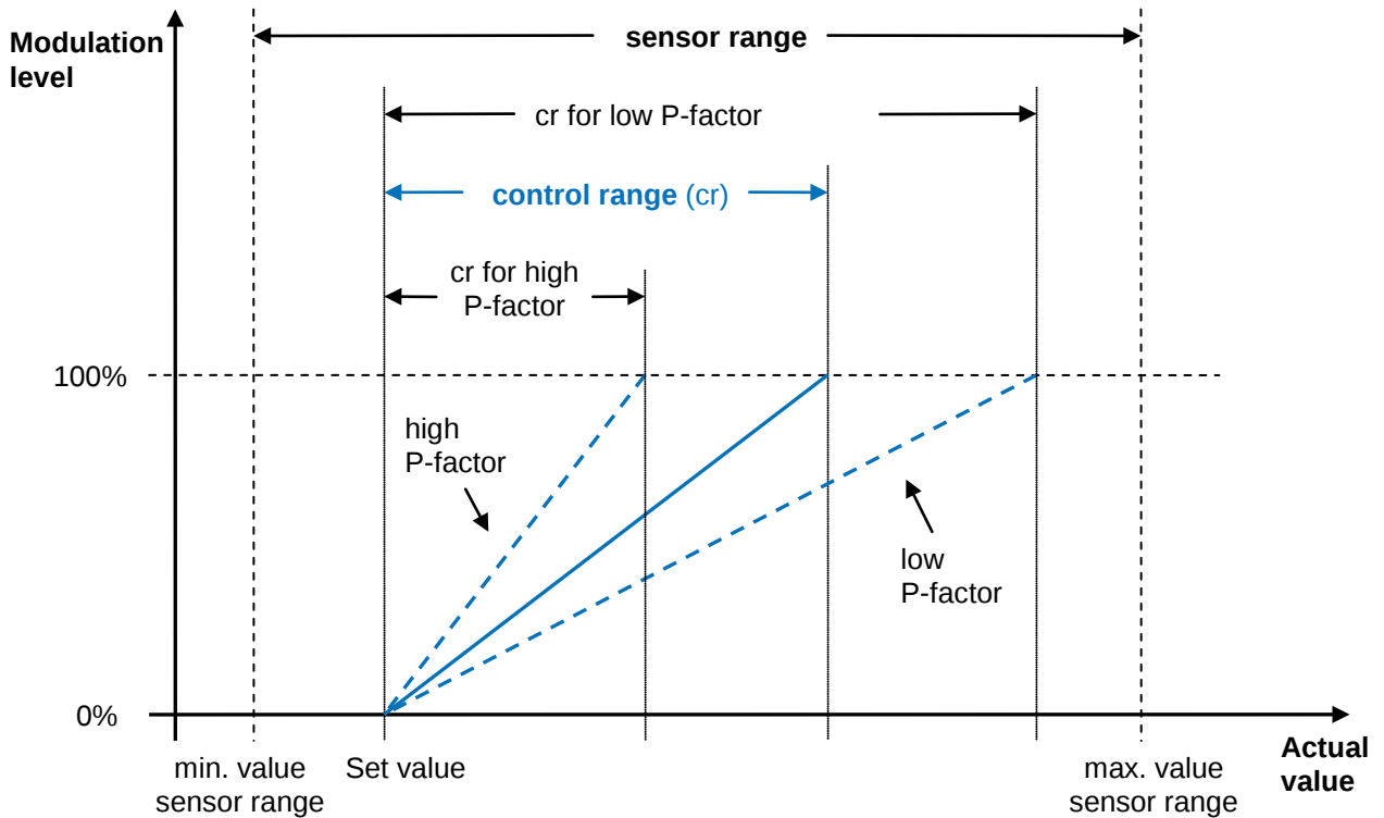
Fig. 7: P-factor
