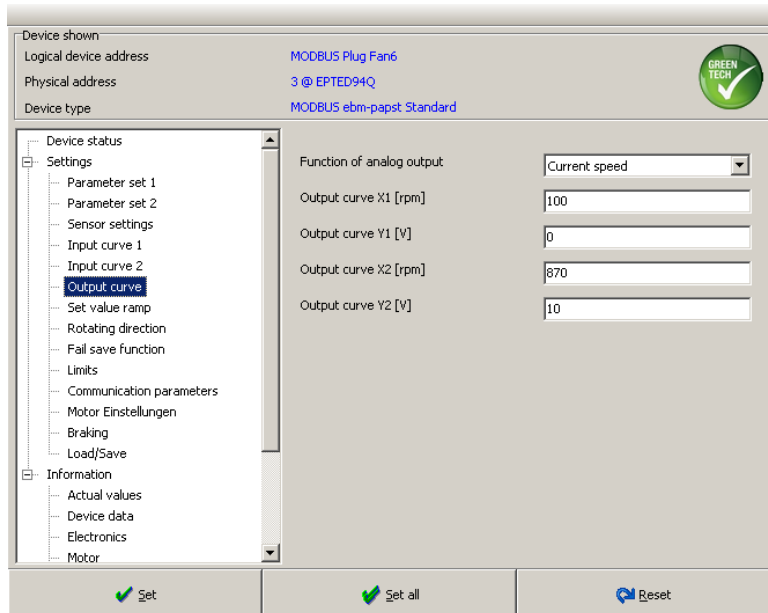
Fig. 35: Output curve
