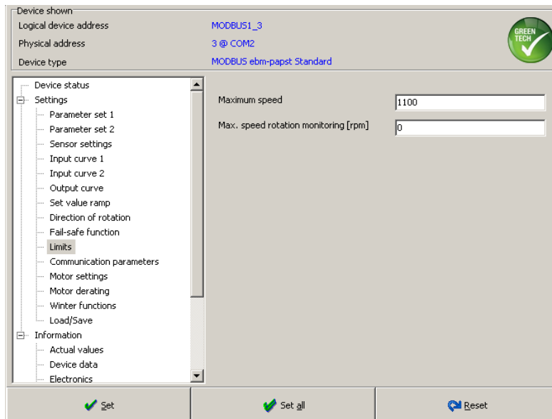
Fig. 40: Parameter set settings for run monitoring
