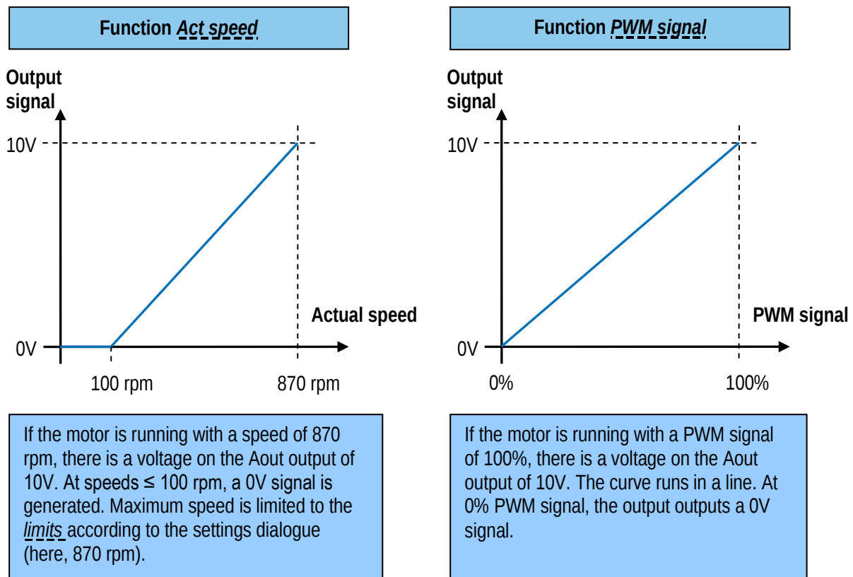
Fig. 36: Output curve
